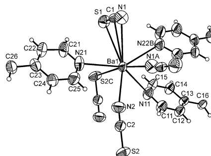
Fig. 7. View of the Ba coordination in compound 3 with labelling and displacement ellipsoids drawn at the 50 % probability level. Symmetry codes A: -x, -y + 1, -z + 1 ; B: x - 1, y + 1, z ; C: -x, -y + 1, -z + 2 . For clarity half of each of the bpe ligands is omitted.
