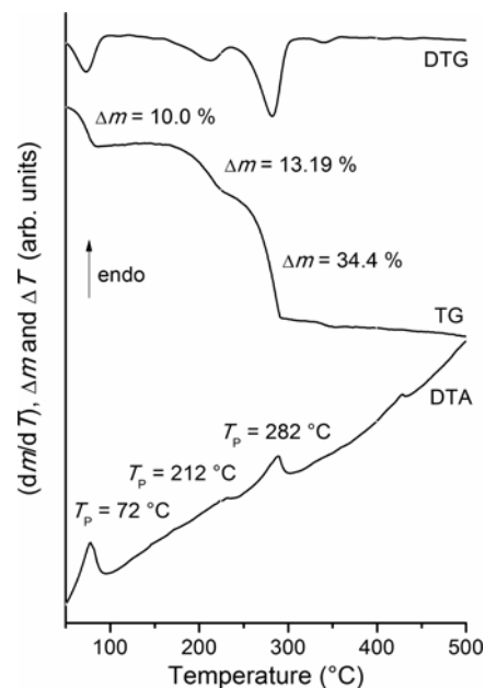
Fig. 12. DTA-TG and DTG curves for compound 1 (given are the mass loss in % and the peak temperatures T_p in °C).
