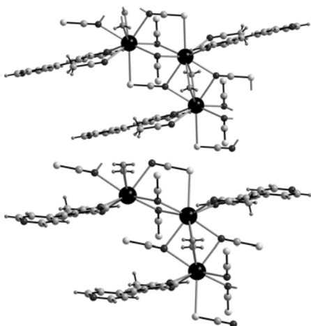
Fig. 10. Part of the chains in the crystal structures of the polymorphs 4I (top) and 4II (bottom). The disorder in 4II is not shown for clarity.
